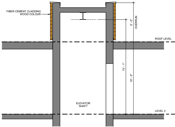
ELEVATOR OVER-RIDE - section
