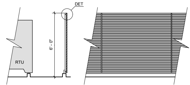
ROOF SCREEN - section/elevation
