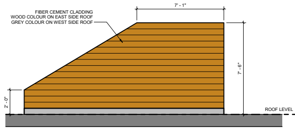
PRIVATE ROOF ACCESS STAIR - elevation
