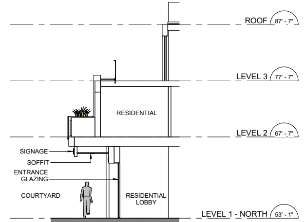
LOBBY ENTRANCE - section
